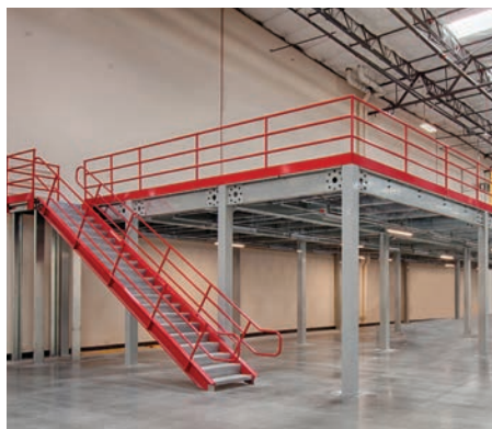
MEZZANINES
